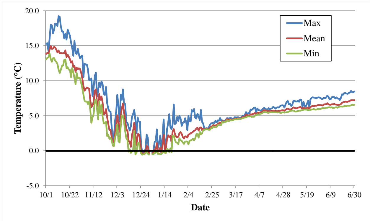
Figure 6. Water temperature ( ^{\circ}\text{C} ) measured at U.S. Bureau of Reclamation Crooked River near Prineville, OR (PRVO) gauge from October 1, 2015 to June 30, 2016. Solid black, horizontal line indicates freezing temperature ( 0^{\circ}\text{C} ).
